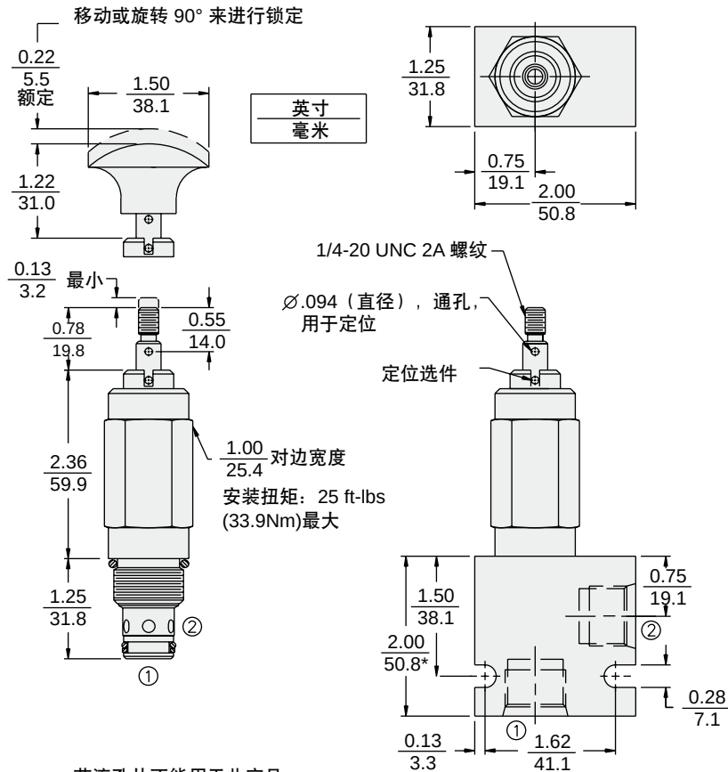
BSP 阀块-55.9
